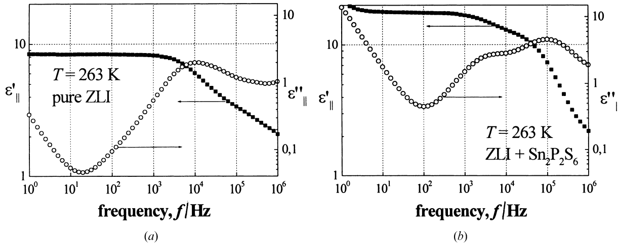
Figure 1. Comparison of \varepsilon'_1 , \varepsilon''_1 for (a) pure LC ZLI-4801-000 and (b) the nematic ferroelectric suspension. Measurements were carried out in the homeotropic cell.
